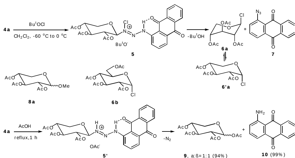
Scheme 5 Oxidation with tert -butyl hypochlorite and acetolysis of a 3-aryl-1-glycopyranosyltriazenes
